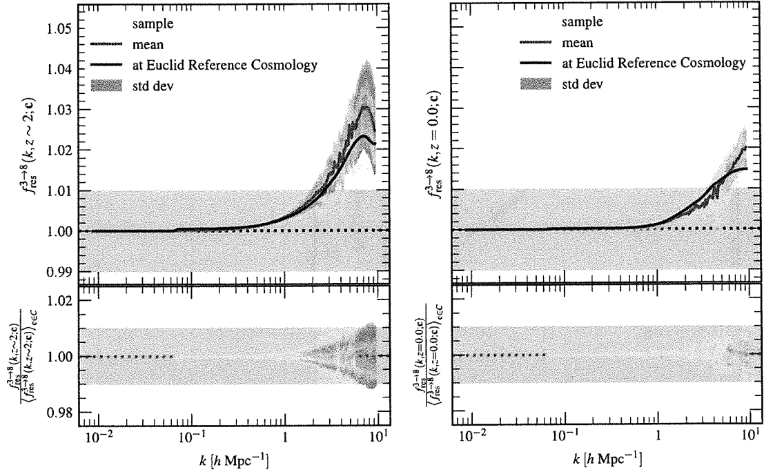
Figure 4. The resolution-induced power suppression is systematic and can be corrected for. In this plot we show the resolution corrections f_{\text{res}}^{3 \rightarrow 8}(k, z; c) computed from a sample of 20 cosmologies represented by the yellow curves. The newly introduced uncertainty due to variance in cosmology, which we neglect, is merely 0.5 per cent (standard deviation, green shaded region) or lower at z = 0 and at the level of 1 per cent at z \sim 2 . Given the fact that the bias itself is at the 5 per cent level at higher redshifts, correcting for the resolution has a positive net effect. The curves corresponding to the Euclid Reference Cosmology are overplotted. We shall use this cosmology to compute the RCF which we apply to all other cosmologies.
