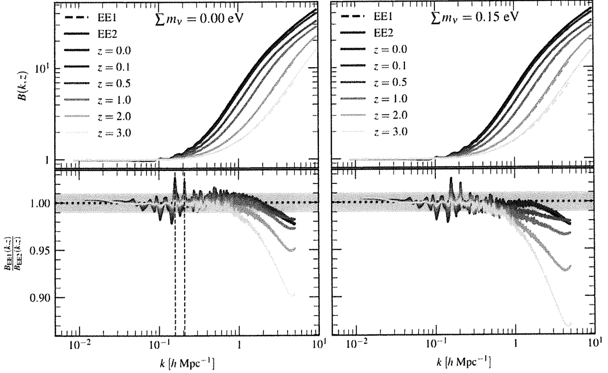
Figure 11. In this figure we compare the NLC prediction of EuclidEmulator2 to that of EuclidEmulator1 for two cosmologies: one for which \sum m_\nu = 0.0 \text{ eV} (left-hand panel) and \sum m_\nu = 0.15 \text{ eV} for the other (right-hand panel). A_s is the same in both cosmologies, however the value of \sigma_8 differs due to the mass difference in the neutrino sector. It is not surprising that the agreement on the largest scales is nearly perfect for both cosmologies as both emulators return values close to unity irrespective of the cosmology by construction. The oscillations around BAO scales are due to cosmic variance. The vertical, black, dashed lines indicate the two k -modes where the curves for EuclidEmulator1 and EuclidEmulator2 deviate the most from each other in Fig. 12. The time-dependent mismatch on small scales is due to the different mass resolutions of the training of the two emulators. A key point is that this plot shows that the agreement between EuclidEmulator1 and EuclidEmulator2 is not only very good for massless neutrino cosmologies where EuclidEmulator1 is supposed to work well by construction, but also for w_0\text{CDM} + \sum m_\nu models which EuclidEmulator1 was not designed for. This suggests that EuclidEmulator1 is able to predict the nonlinear power spectrum within 1 per cent of accuracy for z < 0.5 even if the cosmology contains massive neutrinos (of course, the linear power spectrum must be computed taking the neutrino masses into account).
