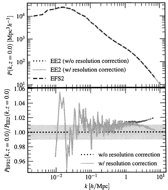
Figure 10. Comparison of full nonlinear power spectra between EFS2 and resolution-corrected product of a CLASS linear power spectrum times an EuclidEmulator2-emulated NLC at the Euclid Reference Cosmology as defined in Table 2. The agreement is generally very good and even at the 1 per cent level or better at small scales. The oscillations at linear scales are expected as EFS2 is not a P+F simulation. We also show the comparison to EuclidEmulator2 when we do not apply the RCF, which shows a clear 2 per cent bias at nonlinear scales.
