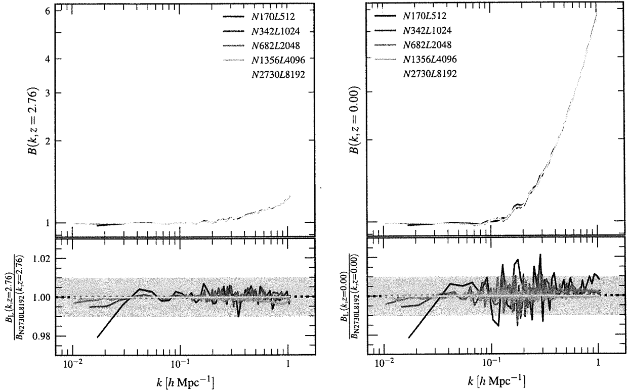
Figure 2. Convergence test results for volume of the NLC factor B(k,z) of simulations with L \in \{512, 1024, 2048, 4096, 8192\} h^{-1} \text{ Mpc} . We show results for two different redshifts. Apart from individual k modes on mildly nonlinear scales, simulation boxes with L = 1024 h^{-1} \text{ Mpc} are converged at the 1 per cent level.
