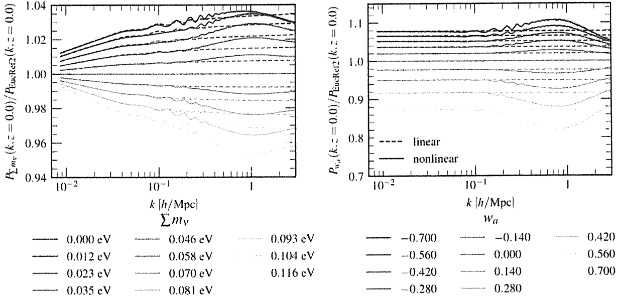
Figure 17. Linear and nonlinear power spectra variation due to varying the cosmological parameters (neutrino mass in the left-hand panel, w_a in the right-hand panel). The power spectra are normalized to the Euclid Reference Cosmology power spectrum. The NLCs for the nonlinear power spectra have been predicted with EuclidEmulator2 in all cases. These plots show clearly that the power spectra differ the most at scales around k \sim 1 h \text{ Mpc}^{-1} .
