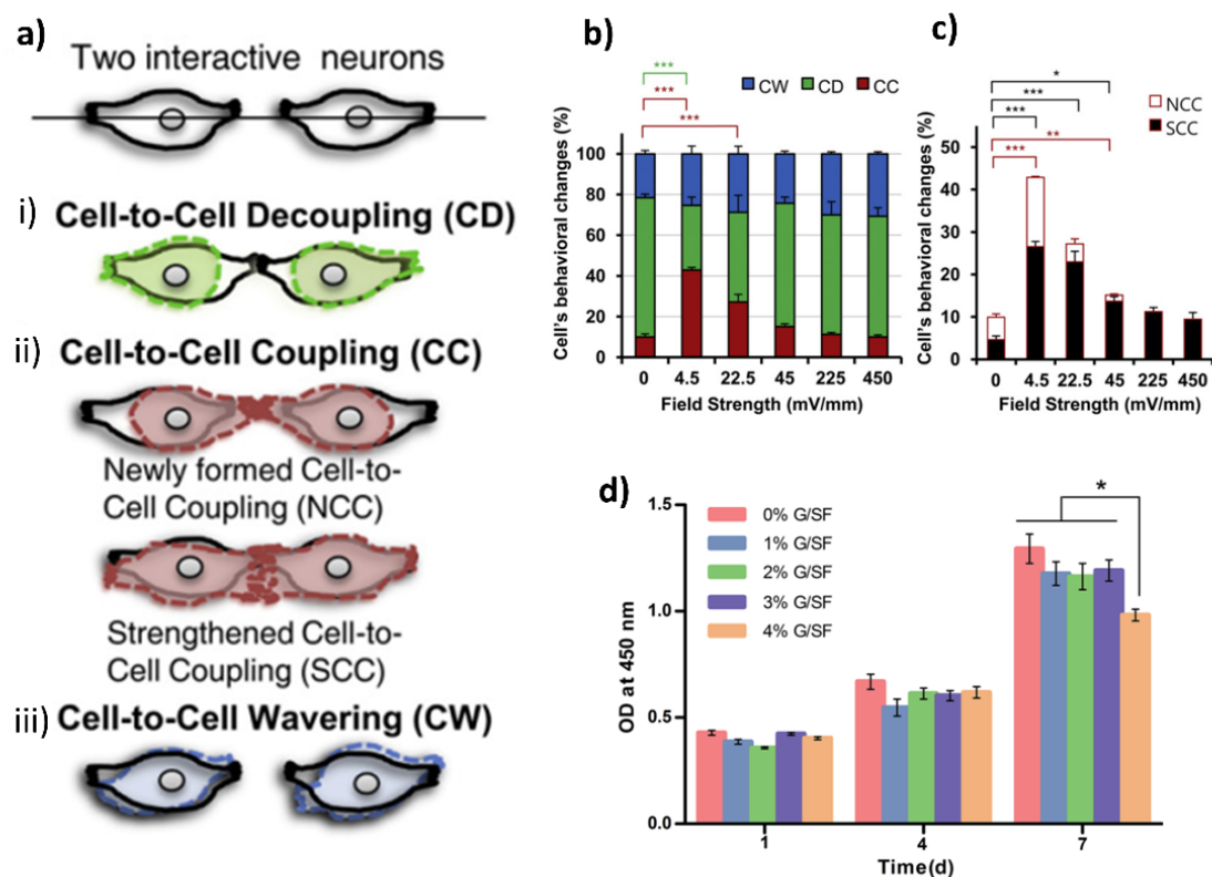
Figure 14. Cell-to-cell interactive reactions to electric field stimulation. (a) , Schematic illustrations of cell-to-cell interactive reactions between two separated cells under electric field stimulation. i) Cell-to-cell decoupling (CD). Cells belonging to the CD group separated from each other after stimulation. ii) Cell-to-cell coupling (CC). The CC group was further classified into two groups: The newly formed cell-to-cell coupling (NCC) group and the strengthened cell-to-cell coupling (SCC) group. The NCC represents a group of cells that respond to electric field stimulation by forming new contacts between cells. The SCC represents a group of cells strengthening existing contacts between cells after electric field stimulation. iii) Cell-to-cell wavering (CW). Cells belonging to the CW group exhibit a wavering behavior following electric field stimulation. Reproduced with permission from ref. [117] . Copyrights 2010 Elsevier, 2017 The Royal Chemical Society. (b) A bar graph categorizing behavioral reactions to electric field strengths. (c) The categorization of CC cells. When we further categorized CC into two groups, there was a clear effect of electric field on NCC; (d) CCK-8 assays of rBMSCs cultured on G/SF fibrous scaffolds. Reproduced with permission from ref. [118] . Copyrights 2010 Elsevier, 2017 The Royal Chemical Society.
