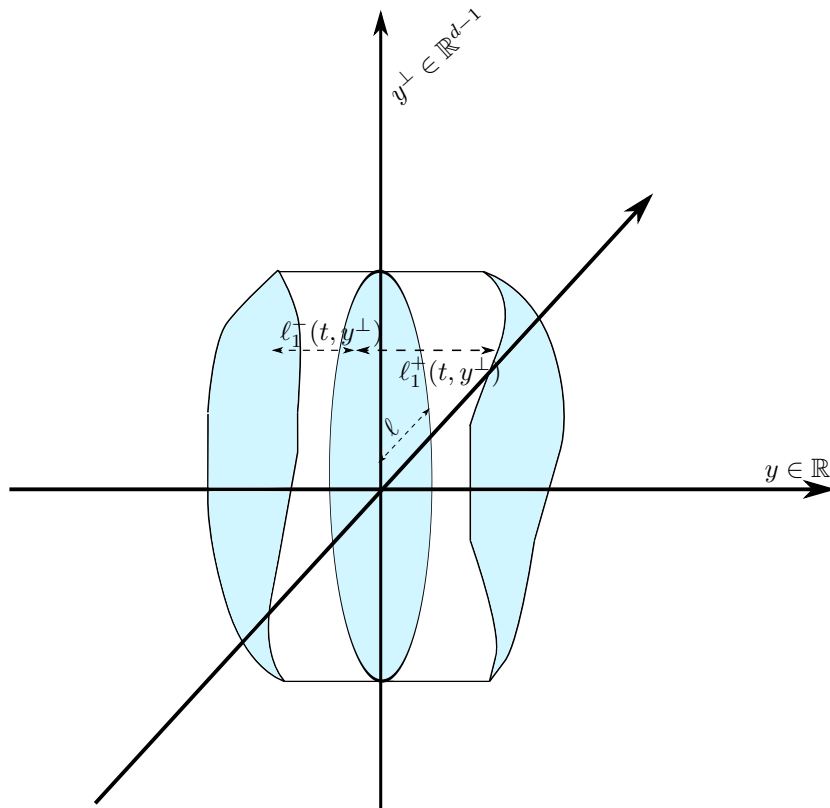
(b) The base of the cylinder at a time t , i.e. the set Q(t) .
