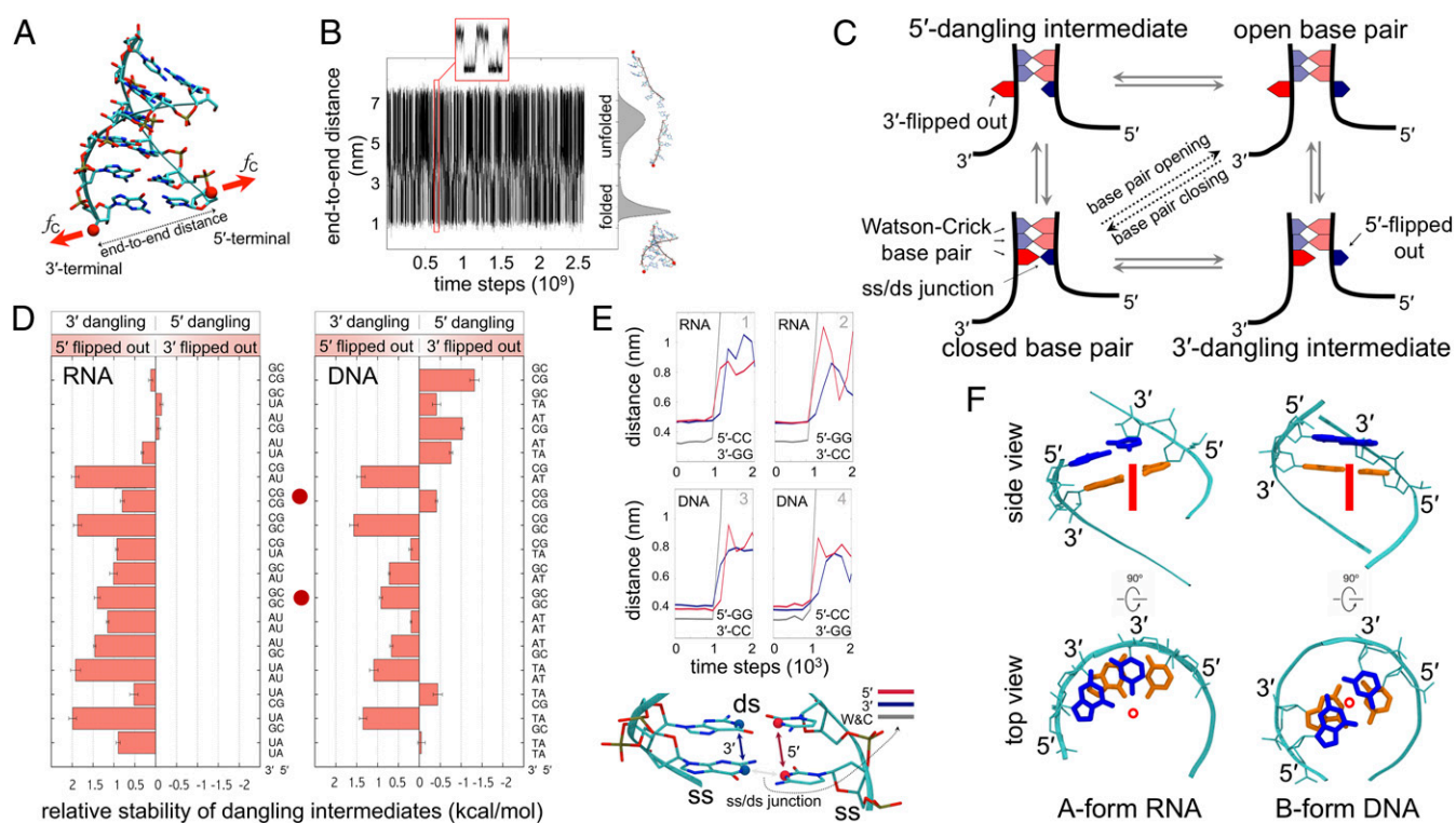
Fig. 1. Modeling the formation and rupture of double helices by mimicking constant-force optical-tweezer experiments (59). (A) Ribbon molecular graphics representation of the ds nucleic acid model and schematic of the reaction coordinate. Red spheres show the 3' and 5' hydroxyl groups of the terminal base pair, defining the end-to-end distance, where the external constant force, f_c , was applied (red arrows; Methods ). (B) Time series of the hopping between folded and unfolded states, zoomed in the red inset. Histogram of the end-to-end distance is on the right, together with sample conformations. (C) Schematic of the stepwise mechanism of base-pair opening/closing. The bases in the ss portion are not shown for sake of clarity. (D) Free-energy difference between the unbiased population of 5'- and 3'-dangling intermediates ( SI Appendix, Methods ) for the base pair at the bottom of each nearest-neighbor combination shown on the vertical axis. Positive values correspond to higher population of 3'-dangling intermediates. Red dots highlight the base-pair combinations explicitly discussed in the main text. Bars indicate SE from bootstrapping (60). (E) Time evolution of the base-pair opening process at a ss/ds junction in RNA and DNA. The distances used to detect W-C pairing (gray), 5'-stacking (red), and 3'-stacking (blue) of the closing base pair are shown. Data are averaged over windows of 300 time steps. (F) Side and top views of adjacent W-C base pairs in RNA and DNA duplexes. The major axis of the helix is shown as a red circle and a red line in the top and side view, respectively. Sugar-phosphate backbone is in cyan sticks and ribbons. Adjacent base pairs are colored in blue and orange to highlight overlap extension.
