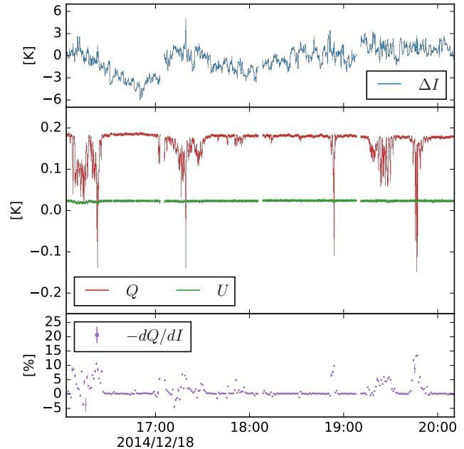
Figure 4. Example timestreams from a single bolometer during a cloudy observation. The top panel shows the Stokes I (intensity) signal, and the middle panel shows demodulated Stokes Q and U polarization signals, with the offsets due to instrumental polarization. The bottom panel shows the slope of the simple linear regression between I and Q , which corresponds to the signed Q polarization fraction.
