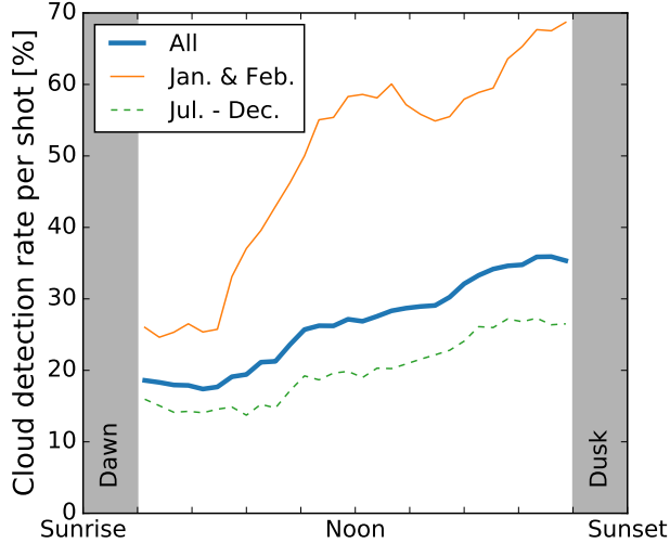
Figure 9. Daytime variation of the cloud detection rate. The horizontal axis represents the time in the daytime, which is scaled with respect to the sunrise and sunset times to adjust their seasonal variations. The blue line shows the result from all the data, and the orange and green lines show the results in the high (January and February) and low (from July to December) seasons, respectively. The shadowed regions show the mask used to cut dawn and dusk.
