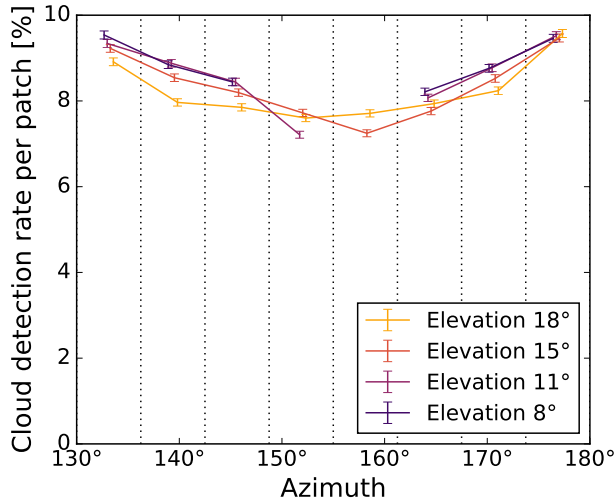
Figure 7. Cloud detection rate for each patch of the sky shown in Fig. 6.
