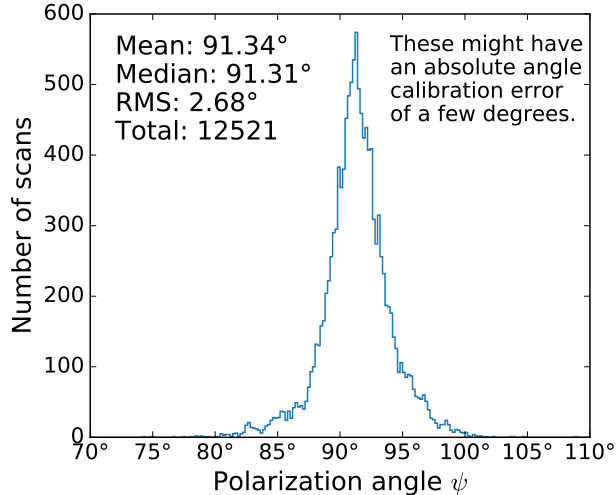
Figure 11. The histogram of the polarization angle of the polarized-burst signal \psi . The mean, median, and root-mean-square (RMS) values are calculated from samples in the range of 70^\circ < \psi < 110^\circ . There are no other bunches outside of the range shown. Note that we have not finalized the absolute angle calibration for this data set yet, and it might have an error of a few degrees.
