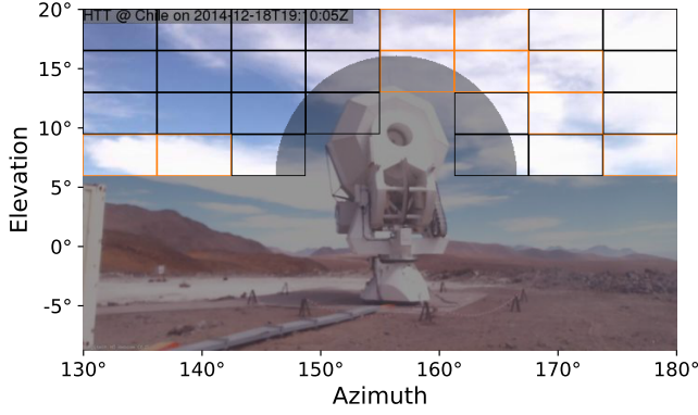
Figure 6. Example of the cloud detection with a webcam image. The shadowed region shows the mask, which is fixed for all the images. The orange and black rectangles show patches with and without cloud detection in this image.
