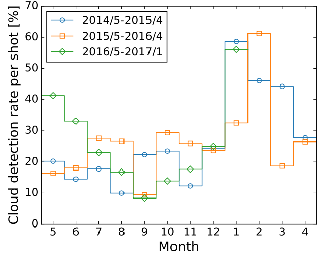
Figure 8. Annual variation of the cloud detection rate. Each line shows the result in the different year. The cloud detection rate increases in January and February every year because of Altiplanic winter.
