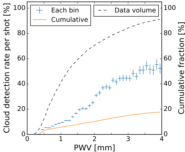
Figure 10. The dependence of the cloud detection rate on the PWV provided by the APEX experiment. Each blue point shows the rate for data in each PWV bin and the orange line shows the rate for all the data below the PWV. The cumulative fraction of the data volume is also shown as the black dashed line.
