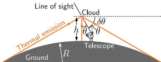
Figure 2. Sketch showing microwave radiation emitted from the spherical ground, reaching a cloud above the observing site.
