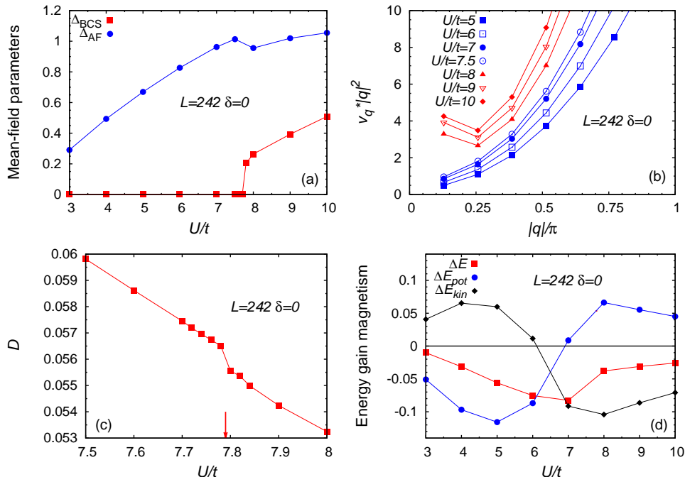
FIG. 2: (Color online) All the simulations shown are performed in the grand-canonical ensemble, at half filling on a L = 242 lattice size. (a): Mean-field variational parameters \Delta_{AF} (blue dots) and \Delta_{BCS} (red squares) as a function of U/t . (b): Fourier transform of the Jastrow factor v(q) , multiplied by |q|^2 , as a function of |q|/\pi , for various values of U/t . The q points are taken on the path in the Brillouin zone connecting \Gamma = (0, 0) to M = (\pi, \pi) . (c): Density of double occupancies D as a function of U/t . The arrow indicates the location of U_{Mott} . (d): Energy gain \Delta E = E_{magn} - E_{nomagn} (red squares), due to the presence of magnetism in the wave function; the potential \Delta E_{pot} = E_{magn}^{pot} - E_{nomagn}^{pot} (blue dots) and kinetic \Delta E_{kin} = E_{magn}^{kin} - E_{nomagn}^{kin} (black diamonds) contributions are also shown.
