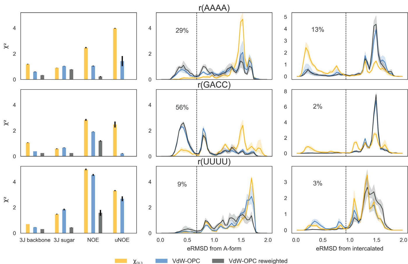
Fig. 4. Comparison between reweighted and unreweighted ensembles for r(AAAA), r(GACC), and r(UUUU) tetranucleotides. (Left) Agreements between calculated and experimental averages for \chi_{0L3} , VdW-OPC, and reweighted VdW-OPC simulations. (Middle) Histograms of eRMSD from ideal A-form. (Right) Histograms of eRMSD from intercalated structure. The dashed lines indicate the thresholds used for calculating the percentage of A-form-like (middle) or intercalated structures (right) upon reweighting.
