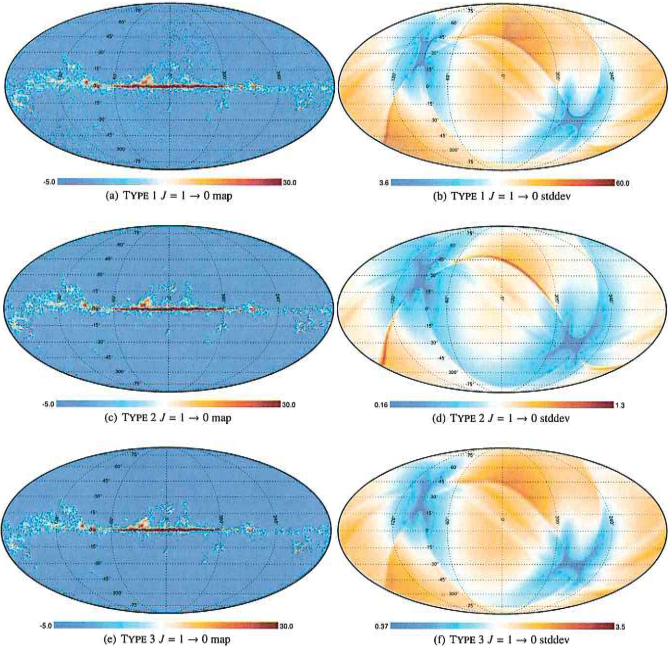
Fig. 3. Full-sky CO J = 1 \rightarrow 0 maps (left) and their respective statistical error maps (right) in \text{K km s}^{-1} units for the three types of Planck CO products. For display purposes only, the TYPE 1 and TYPE 3 maps are smoothed to 15' to ease the comparison to the TYPE 2 maps. The error maps correspond to the non-smoothed product. The maps are in Galactic coordinates and follow the HEALPix pixelization scheme for N_{\text{side}} = 2048 .
