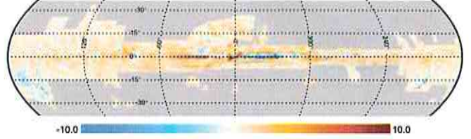
Fig. 11. Residual map with respect to the Dame et al. (2001) map in \text{K km s}^{-1} for the TYPE 1 J = 1 \rightarrow 0 Planck CO map. The Planck maps have been recalibrated to Dame before performing the subtraction.
