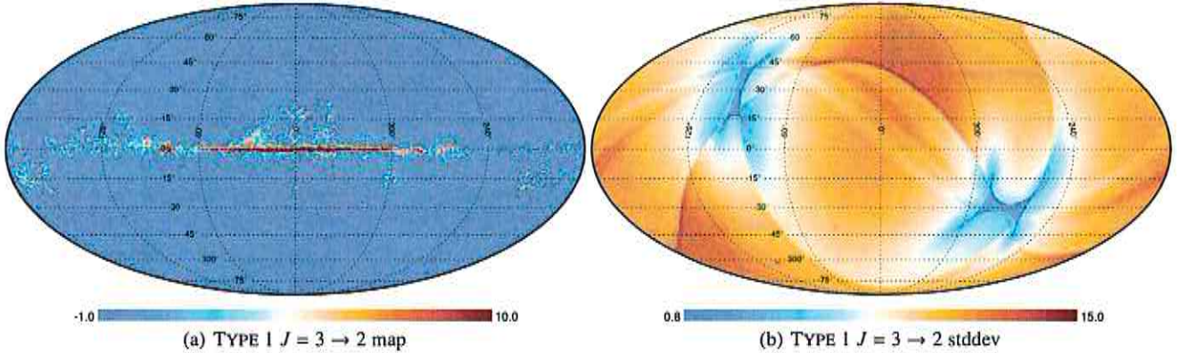
Fig. 5. TYPE 1 full-sky CO J=3 \rightarrow 2 maps (left) and its statistical error map (right) in \text{K km s}^{-1} units. The map has been smoothed to 15' for display purpose but the error map corresponds to the non smoothed product. The maps are in Galactic coordinates and follow the HEALPIX pixelization scheme for N_{\text{side}} = 2048 .
