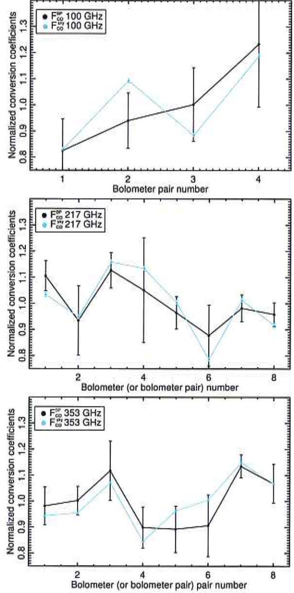
Fig. 2. Comparison of normalised CO conversion coefficients computed from the bandpass measurements (black) or estimated on the sky (blue) for the 100 ( top ), 217 ( middle ) and 353 GHz ( bottom ) channels. See Table 2.
