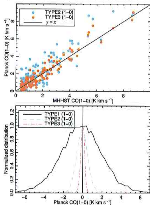
Fig. 17. Comparison of the Planck CO(1 \rightarrow 0) maps with the high Galactic latitudes CO detections and non detections from MHHST00. Top : correlation between the CO detections in MHHST00 and the Planck TYPE 2 and TYPE 3 maps. The latter was first smoothed to 15'. Bottom : distribution of all Planck CO(1 \rightarrow 0) maps (at 15' resolution) at the non-detection positions of MHHST00. The width of the distribution is compatible with the noise in the maps. Differences with respect to the values in Table 3 can be explained by the inhomogeneities of the noise in the Planck maps.
