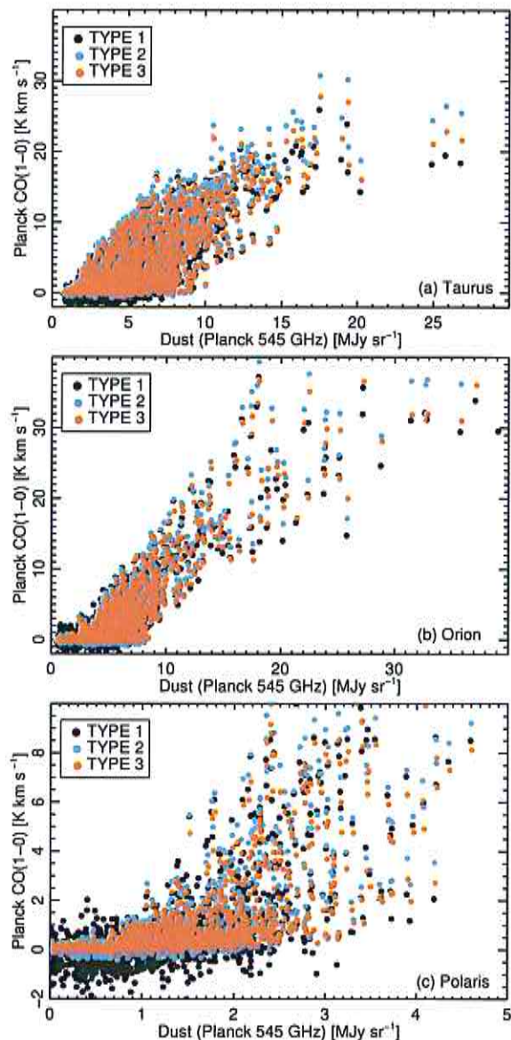
Fig. 6. Comparison of the 3 types of CO products with a dust template map for the Taurus (top), Orion (middle) and Polaris (bottom) molecular clouds.
