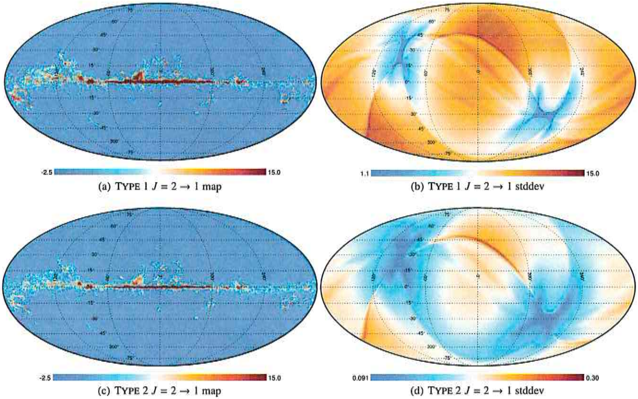
Fig. 4. Full-sky CO J=2 \rightarrow 1 maps (left) and their respective statistical error maps (right) in \text{K km s}^{-1} units for TYPE 1 (top) and TYPE 2 (bottom) Planck CO products. The TYPE 1 map has been smoothed to 15' for display purposes but the error map corresponds to the non smoothed product. The maps are in Galactic coordinates and follow the HEALPIX pixelization scheme for N_{\text{side}} = 2048 .
