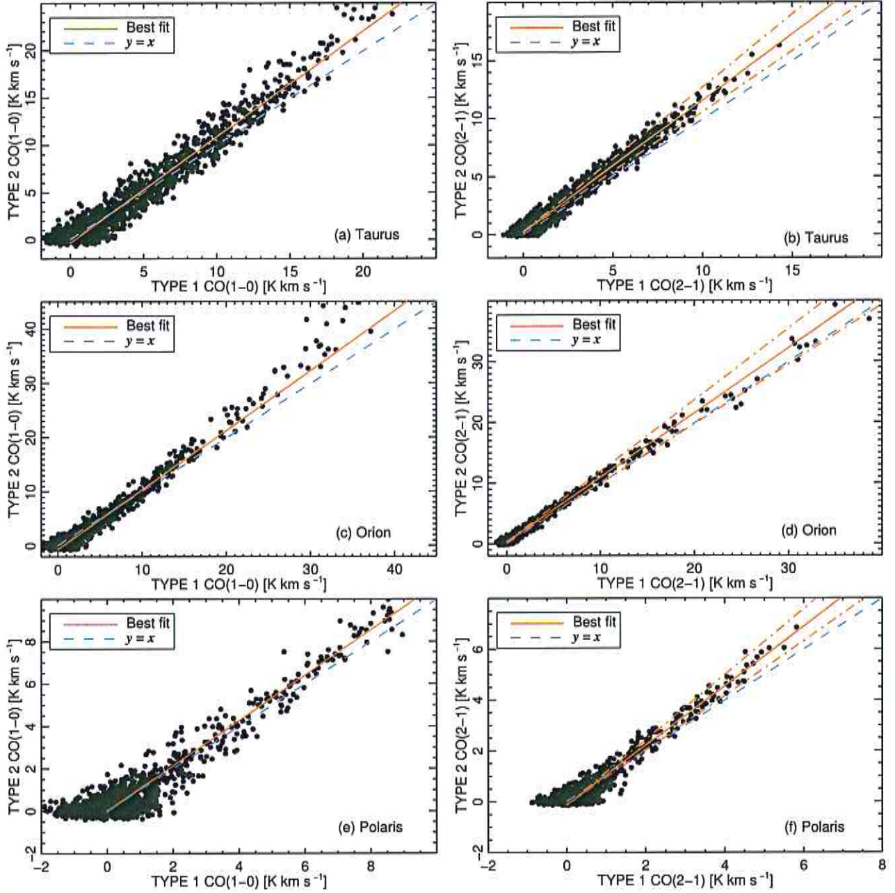
Fig. 9. Correlation between TYPE 1 and TYPE 2 CO maps at 115 GHz (left column) and 230 GHz (right column) in the Taurus (top), Orion (middle) and Polaris (bottom) molecular clouds. The best linear fits (orange solid line) have been computed between 2 and 15 \text{K km s}^{-1} at 115 GHz and between 1 and 15 \text{K km s}^{-1} at 230 GHz, where bulk of the data lie and avoiding the noise around zero. The best-fit slopes and uncertainties are: a) 1.12 \pm 0.03 ; b) 1.14 \pm 0.01 ; c) 1.10 \pm 0.04 ; d) 1.07 \pm 0.01 ; e) 1.07 \pm 0.06 ; and f) 1.17 \pm 0.04 . The intercepts are compatible with zero within error bars. The orange dot-dashed lines in the bottom panels correspond to the recalibration uncertainty due to the contribution of the J = 3 \rightarrow 2 line in the TYPE 2 J = 2 \rightarrow 1 product. See text for detail.
