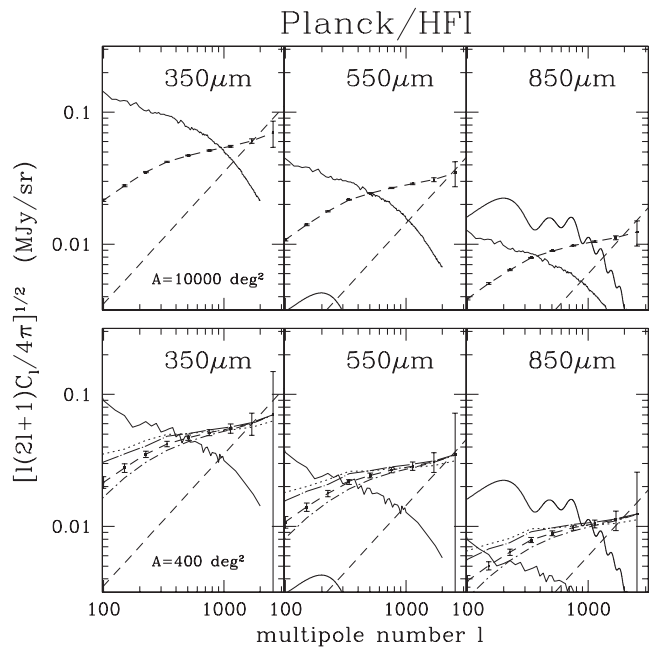
Figure 10. Power spectra of background fluctuations due to clustering of protospheroidal galaxies below the detection limit in the high frequency Planck/HFI surveys (points with error bars for bins \Delta\ell = 0.4\ell ) compared with the power spectra of the diffuse Galactic dust emission (broken lines), of Poisson fluctuations due to extragalactic point sources below the detection limits (dashed lines), and of the CMB (solid line, visible in the 850-μm panel, and in the bottom left-hand corner of the 550-μm panel). The dust power spectra are based on the Finkbeiner et al. (1999) model; the upper set of panels refer to the \simeq 9650 deg 2 at |b| > 50^\circ , the lower set refers to the 400-deg 2 low-dust region centred at l \simeq 245^\circ , b \simeq -50^\circ . In the bottom panels, we show, in addition to the predicted power spectrum for our reference cosmological model, with \Omega_m = 0.3 and \Omega_b = 0.047 (dashed line), the effect of different choices of these two parameters: \Omega_m = 0.15 and \Omega_b = 0.045 (dotted line); \Omega_m = 0.27 and \Omega_b = 0 (dot-short dashed line); \Omega_m = 0.27 and \Omega_b = 0.09 (dot-long-dashed line).
