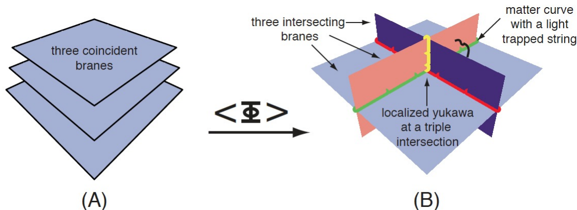
Figure 1. A configuration of intersecting branes can be studied as a background in a theory of coincident branes. In (A) we have a stack of three branes supporting a U(3) gauge group. In (B), the Higgs field \Phi develops a vev and describes three intersecting branes with gauge group U(1)^3 . At the intersection of branes are trapped charged fields. At triple intersections a Yukawa coupling is generated.
