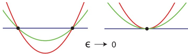
Figure 2. The Yukawa behaves continuously with respect to deformations of the background parameters. On the left we have three matter curves, illustrated by the colored lines, meeting transversally at two points leading to a rank two superpotential. On the right a parameter \epsilon \rightarrow 0 and the Yukawa points collide leading to a rank two contribution from a single intersection.
