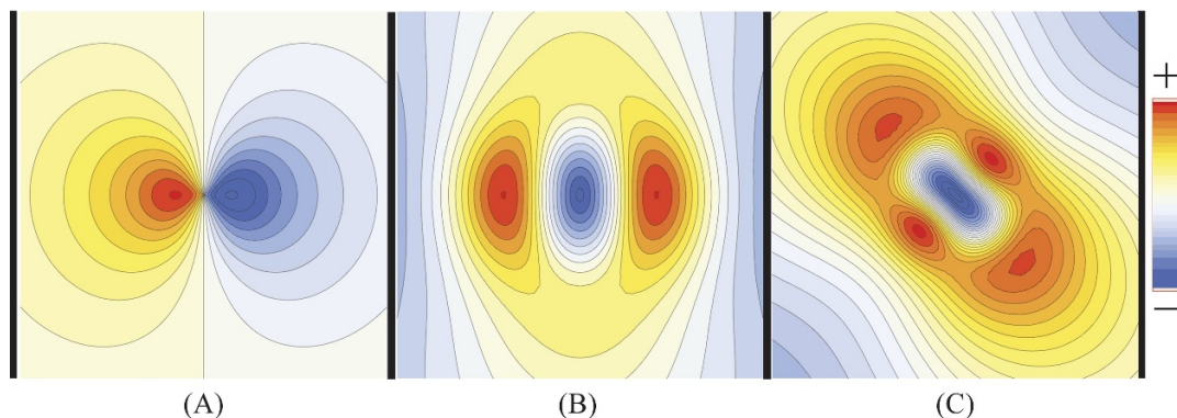
Figure 3. Contour plots of the distorted bulk mode \varphi in the background (3.18) with nontrivial \mathbb{Z}_2 monodromy. The images show the profile of the zero modes in the complex x plane centered on the branch locus. The complex coordinate y is suppressed. Figure (A) shows the upper-right entry of \varphi while (B) and (C) illustrate the real and imaginary parts of the lower-left entry of \varphi .
