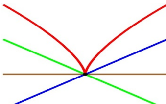
Figure 5. The local geometry of the E_8 point with \mathbb{Z}_2 \times \mathbb{Z}_2 monodromy specified by the background (7.24). The \bar{\mathbf{5}}_H curve, depicted in red, has a cusp singularity at the origin. The remaining matter curves are smooth and meet transversally.
