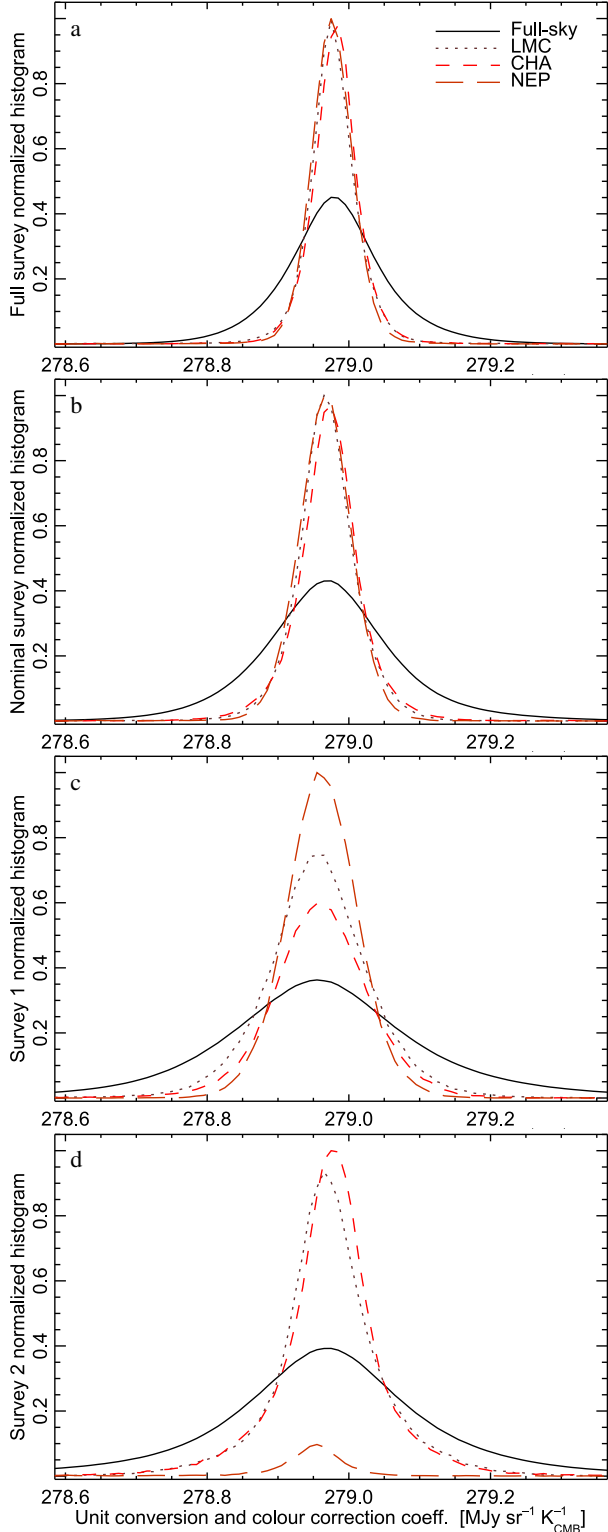
Fig. 27. Histograms of the 353 GHz combined unit conversion and dust colour correction maps corresponding to the Full survey a ), Nominal survey b ), survey 1 c ) and survey 2 d ) data. The plots include histograms based on the full sky as well as the LMC, CHA, and NEP regions.
