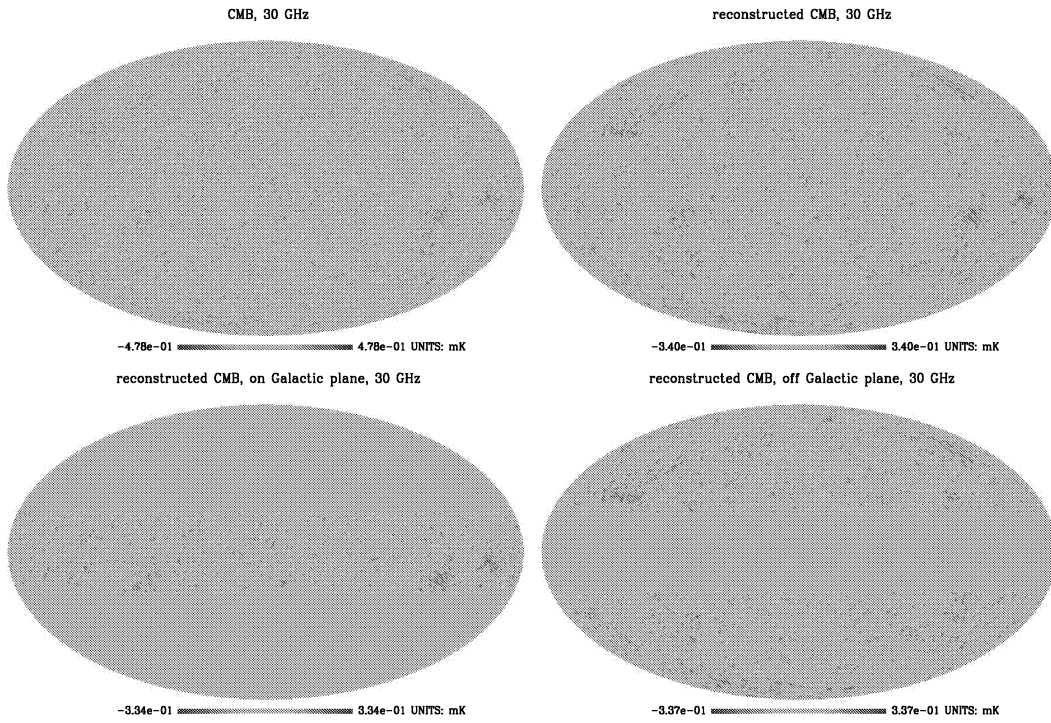
Figure 4. Input (top-left) and output CMB maps for case 1, at 30 GHz.
