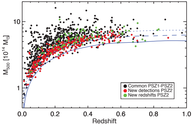
Fig. 14. M_{500}-z plane distribution of the 1093 PSZ2 clusters with known redshift. New PSZ2-detected clusters are indicated by red dots, while common PSZ1 and PSZ2 clusters are indicated by black dots. Green dots mark the common PSZ2–PSZ1 detections with updated redshifts in PSZ2. The solid, dashed, and dotted lines indicate the limiting mass at 20%, 50%, and 80% survey completeness, respectively.
