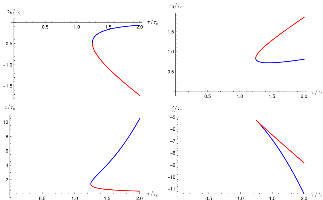
Figure 11. Plot of the solutions of (6.24) for \mathcal{B} = 1.1\mathcal{B}_c , together with the corresponding energy \epsilon and Helmholtz free energy f densities.
