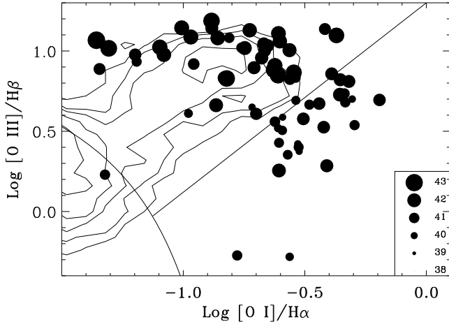
Fig. 2. \log [\text{O III}]/\text{H}\beta versus \log [\text{O I}]/\text{H}\alpha diagram only for sources with L_{[\text{O III}]} > 10^{40} \text{ erg s}^{-1} : contour lines represent the SDSS sample while black circles indicate the 3CR sources. The symbol size increases with [\text{O III}] luminosity. As in Fig. 1, the curved line divides the star-forming galaxies and AGN, while the oblique line divides Seyferts and LINERs (according to K06).
