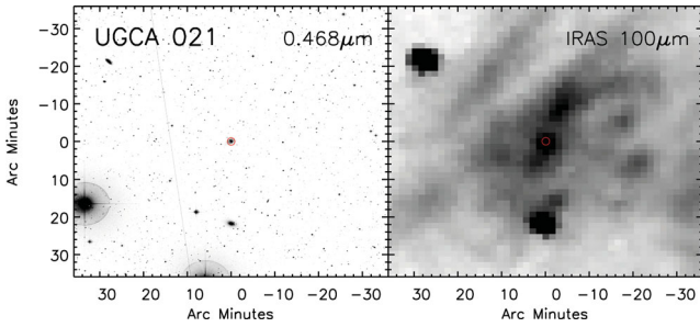
Figure 4. Postage stamp image of the galaxy UGCA-021 ( z = 0.006622 ), at 0.468 \mu\text{m} (left-hand panel) and at 100 \mu\text{m} (right-hand panel). This galaxy, indicated by the red circle, is flagged as extended in the ERCSC at 545 GHz and has CIRRUS=0.094. However the IRAS map shows that it lies behind a prominent structure in the Galactic interstellar medium.
