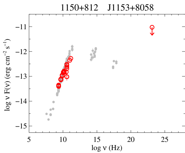
Fig. 69. 1150+812.
