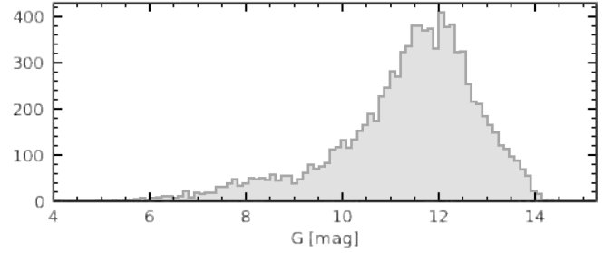
Fig. 7. G -band brightness distribution of the FPR sample.
