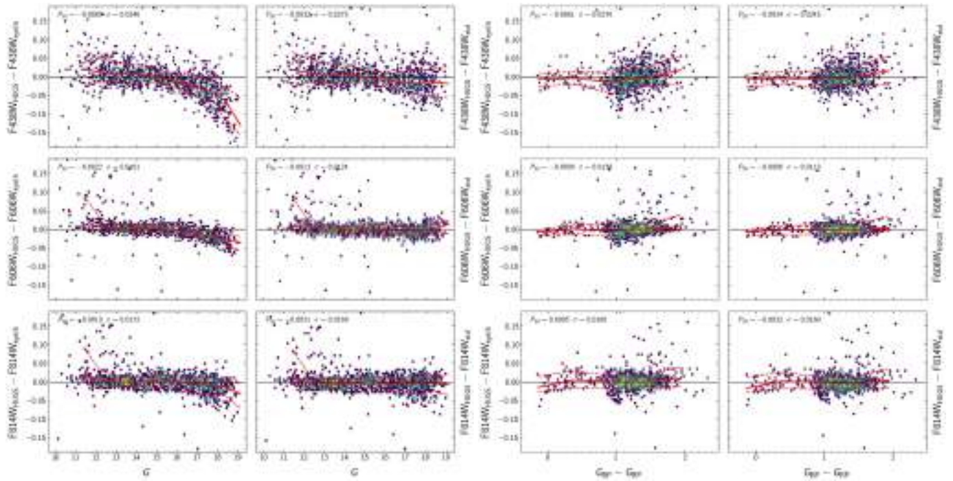
Fig. G.5. Performance and standardisation of HST F438W_{WFC3/UVIS} , F606W_{ACS/WFC} , and F814W_{ACS/WFC} bands XP synthetic magnitudes using the reference sample described in Sect. 3.5. The arrangement of the plots and symbols are the same as Fig. G.1, above.
