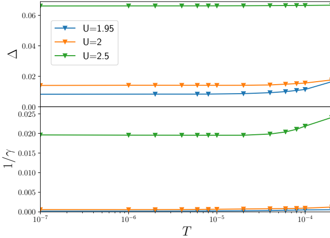
FIG. 8. Temperature dependence of the parameters \Delta and \gamma in Eq. (58) fitted through NRG results at \epsilon_d = 0.1 and different U > U_c . We note that both \Delta^2 and 1/\gamma vanish approaching U_c , although 1/\gamma \ll \Delta^2 .
