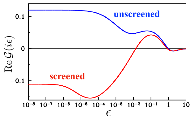
FIG. 5. \text{Re}\mathcal{G}(i\epsilon) versus the Matsubara frequency \epsilon at \epsilon_d = 0.1 in the screened phase, U = 1.75 red curve, and in the unscreened one, U = 2 blue curve.
