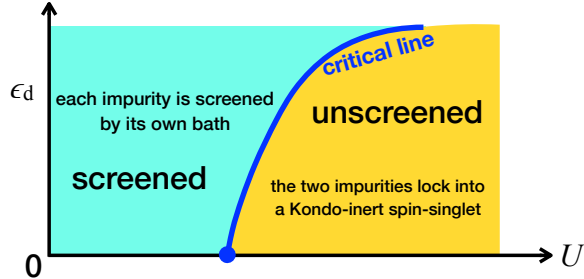
FIG. 4. Phase diagram of the impurity model (48) at fixed hybridisation width \Gamma and J \ll \Gamma , as function of U and \epsilon_d > 0 . The case \epsilon_d < 0 is symmetric.
