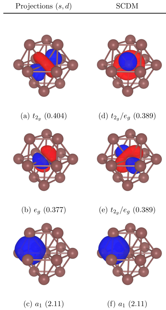
Fig. 2 MLWFs obtained by Wannierising the s - d complex in copper. First column: three representative MLWFs obtained from using atomic orbital projections to define the initial subspace (see main text for description). Panel (a) shows one of the three MLWFs with t_{2g} character; panel (b) shows one of the two MLWFs with e_g character; panel (c) shows one of the two broad s -like orbitals centred on a tetrahedral-interstitial site. Second column: three representative MLWFs obtained from using SCDM to define the initial subspace. Panels (d) and (e) show two of the five MLWFs with mixed t_{2g}/e_g character; panel (f) shows one of the two broad s -like orbitals centred on an tetrahedral-interstitial site. Below each function its individual spread in \text{Å}^2 is reported. Isosurfaces are plotted with an isovalue of \pm 0.45 \text{ Å}^{-3/2} .
