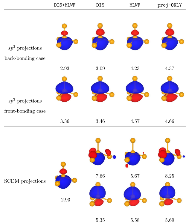
Fig. 1 Wannier functions obtained by Wannierising the four valence bands plus the four low-lying conduction bands in silicon. First row: the initial subspace is defined by projecting the Bloch states \psi_{n\mathbf{k}}(\mathbf{r}) on eight appropriately oriented sp^3 -type orbitals giving back-bonding (BB) MLWFs in all cases. Second row: as above but with different orientations for the sp^3 -type orbitals, resulting in front-bonding (FB) MLWFs in all cases. Third row: the initial subspace is obtained from the SCDM method. Here, the eight sp^3 -type WFs are in the BB configuration only when a full minimisation is performed. In all other cases, a mixture of configurations is obtained instead. The values below each WF isosurface (isovalue = \pm 0.45 \text{\AA}^{-3/2} ) is the value of the individual spread in \text{\AA}^2 .
