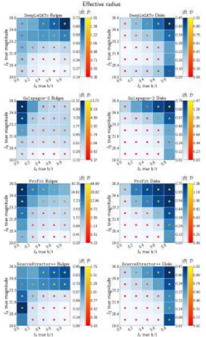
Fig. 9. Absolute bias |\mathcal{B}| and dispersion \mathcal{D} for the effective radius of bulge (left column) and disc (right column) components in the double-Sérsic simulation, as a function of bulge-to-total ratio ( x -axis) and apparent I_E magnitude ( y -axis). Each row shows a different code. For ProFit and Galapagos-2, the colour scale is logarithmic. In each panel, the colour of the squares is proportional to the mean bias \mathcal{D} (lighter being smaller), and the colour of the dot inside each square indicates the dispersion \mathcal{D} (redder being lower). For most of the codes, we find the expected behaviour: both the bias and the dispersion increase for faint objects, as well as at small b/t for bulges and large b/t for discs.
