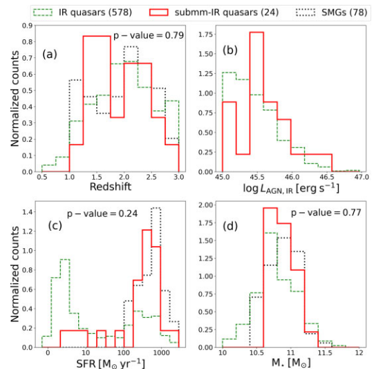
Figure 1. Normalized distributions for the full IR quasar sample (578 sources) of A22 (green dashed), the 24 IR quasars with ALMA sizes (red solid), and the control sample of 78 SMGs (black dotted). In three panels, the KS p-value between the IR quasars with sizes and the SMGs is quoted. (a) redshifts; (b) 8–1000 \mu\text{m} AGN luminosity (c) SFRs; (d) stellar masses.
